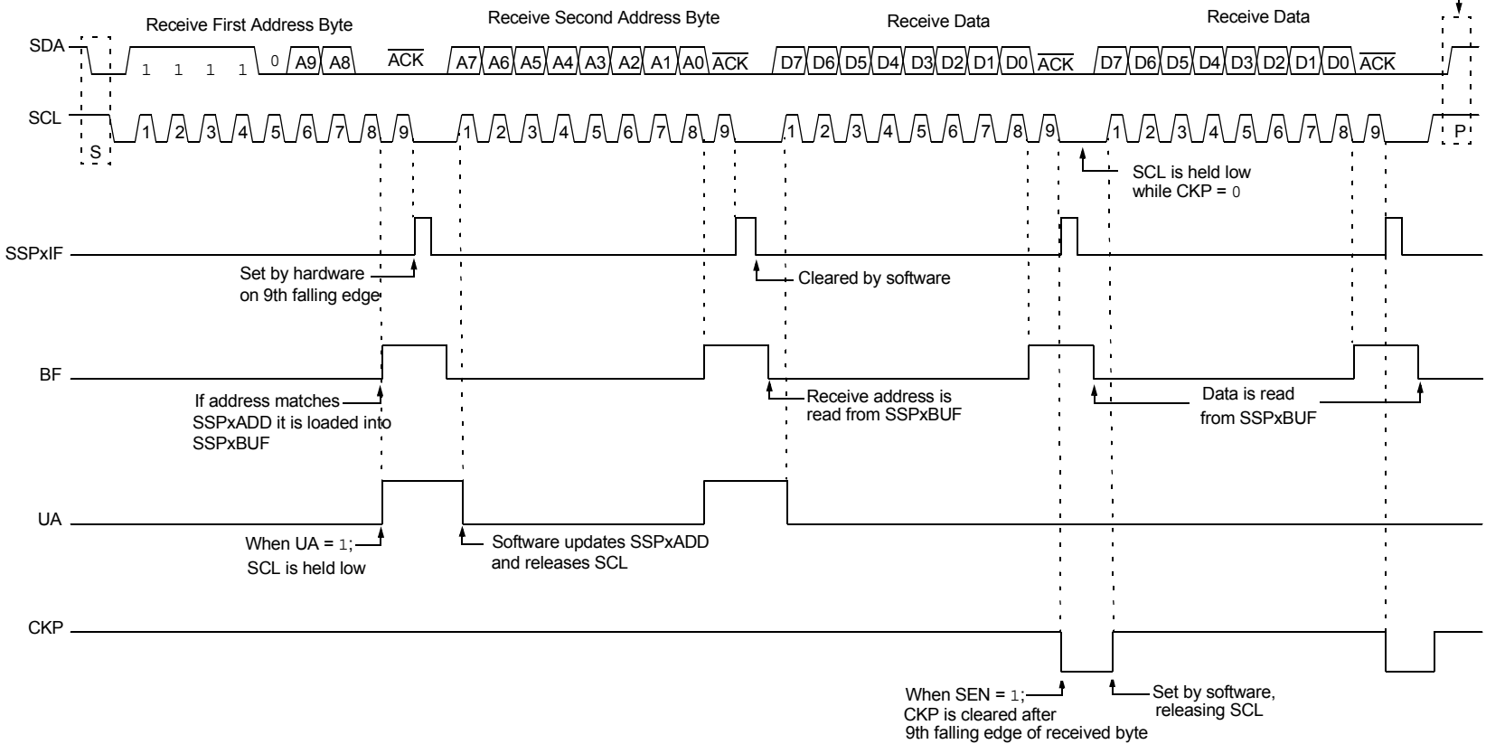
Master sends Stop condition
